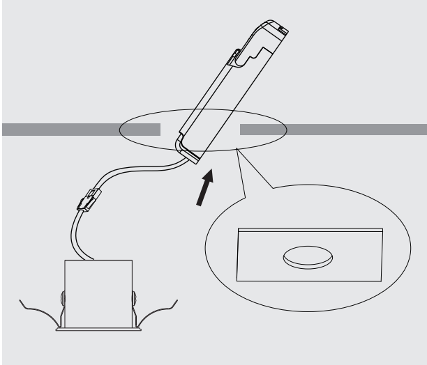
1. Cut out opening on the ceiling accordingly.
