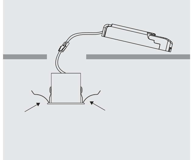
2. Compress the spring clips and insert luminaire into the ceiling opening.
